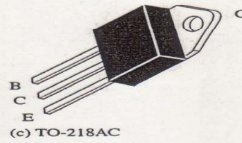
(c) TO-218AC
